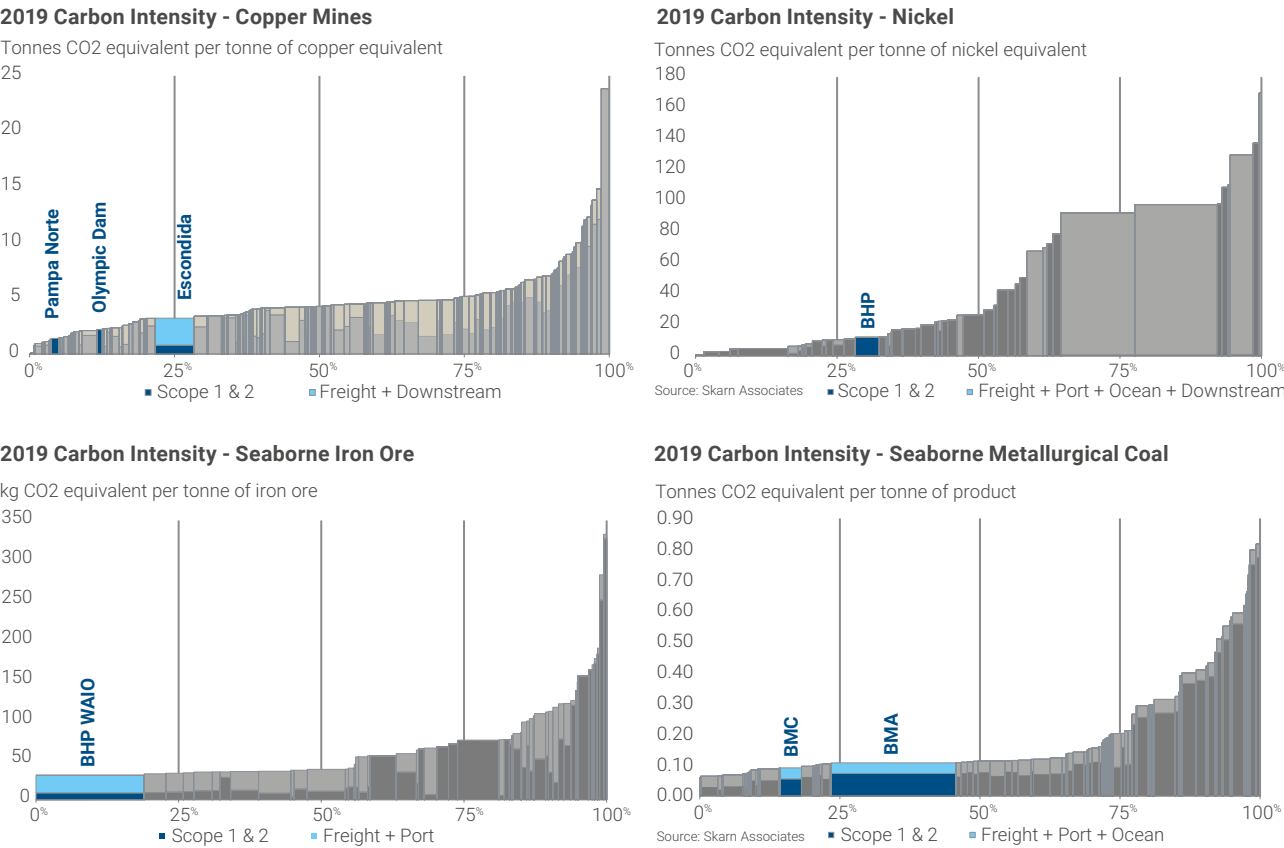
Figure 14: Operational emissions vary widely across assets and across commodities
