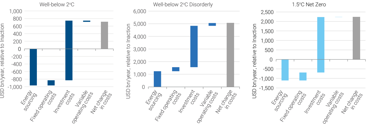
Figure 9: Scenario costs
