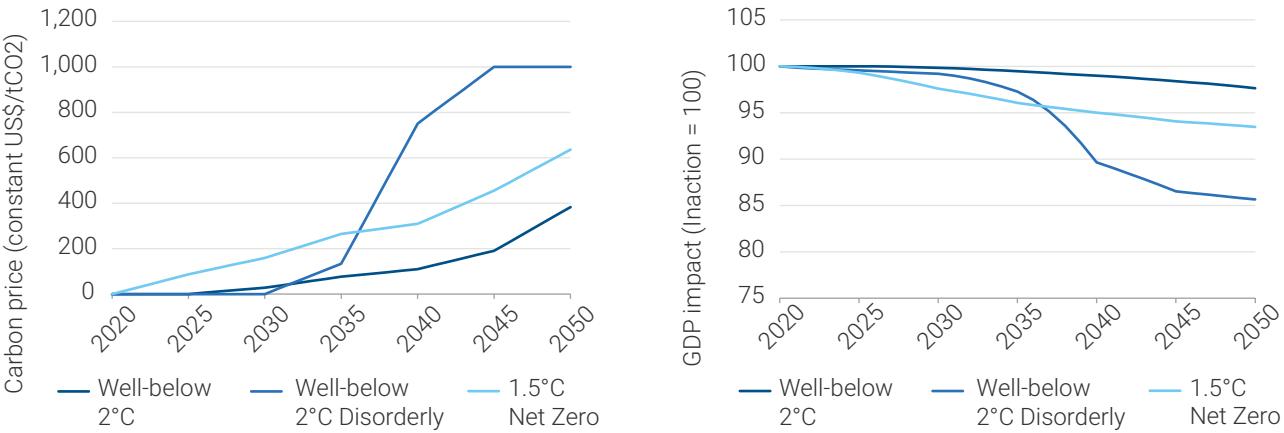
Figure 8: Scenario impacts
