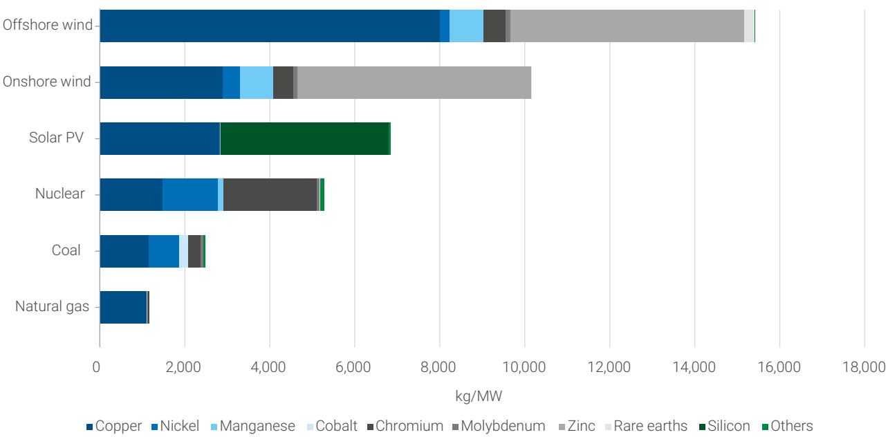
Figure 13: Mineral intensity of clean and conventional power generation technologies
