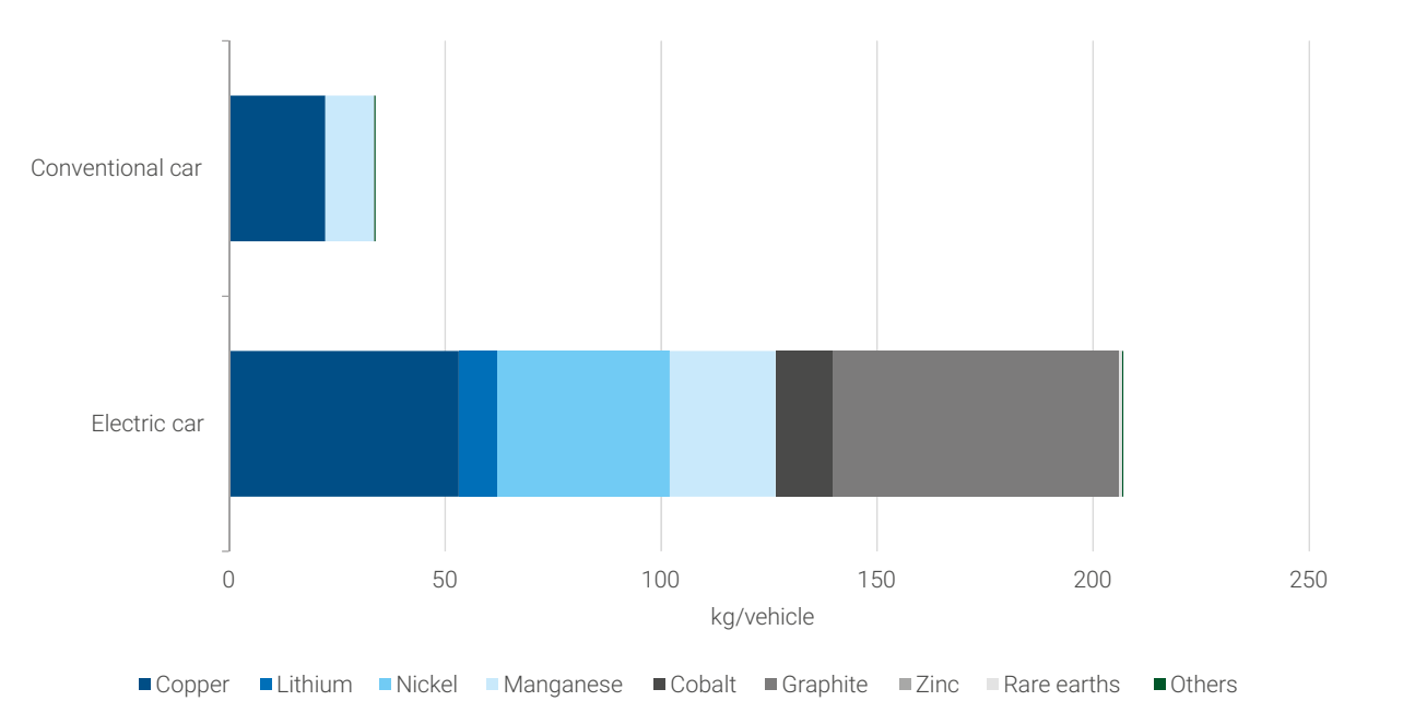
Figure 12: Mineral intensity of electric and conventional cars
